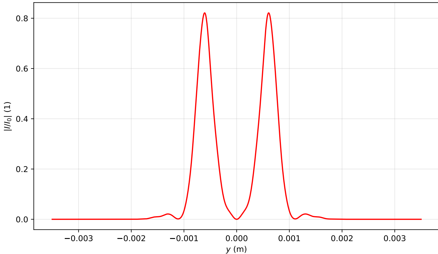
Intensity profile I(x=0, y, z=1.115)/I_0 , P_{in}=6.0P_{cr} , artificial time
